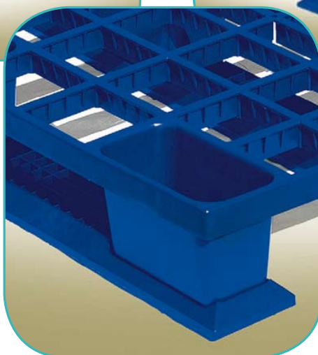
PPS80 1200 X 800 X 145 mm 2500 kg / 1200 kg Non encastrable / 3 patins
