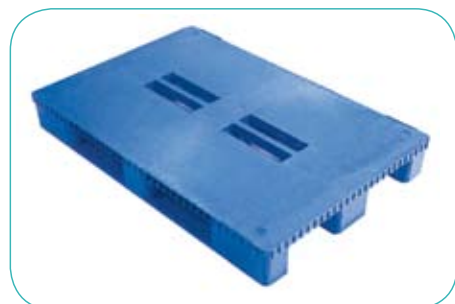
EP1208 1200 X 800 X 160 mm 6000 kg / 1000 kg / 800 kg
