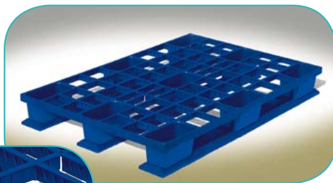
PPS80 1200 X 800 X 145 mm 2500 kg / 1200 kg Non encastrable / 3 patins
